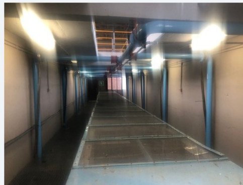
COVERED PROCESS CHANNEL AND DISTRIBUTION PIPEWORK
