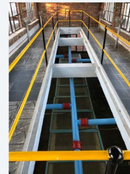
PROCESS CHANNEL, PIPEWORK AND GUARDED ACCESS
